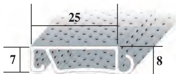
FBS 2025 WIND
