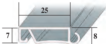
FBS 2025
